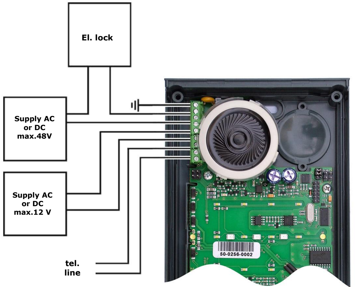
Lock and Backlight Connection
