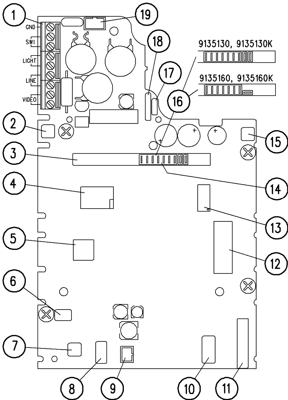
Fig.: PCB Layout, Version 10
